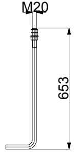
4 x M20 x 720 Anchor Bolts
