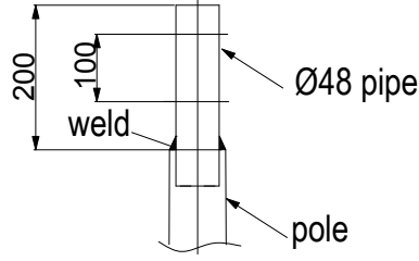
C-C Section
