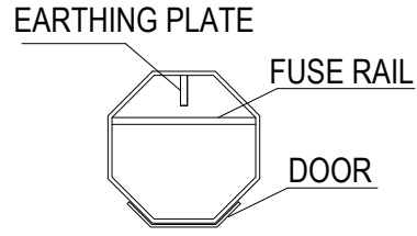
B-B Section
