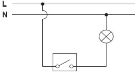
Circuit Diagram for Switch
