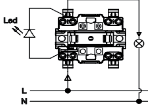
Circuit Diagram for Switch
