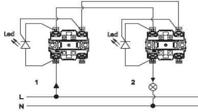
Circuit Diagram for Switch
