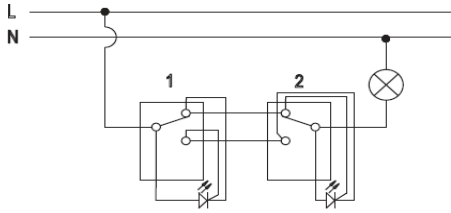
Circuit Diagram for Switch
