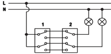
Circuit Diagram for Switch
