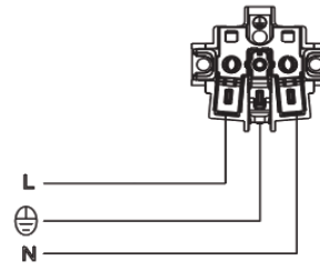
Circuit Diagram for Socket
