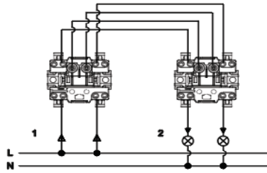
Circuit Diagram for Switch
