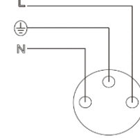
Circuit Diagram for Socket
