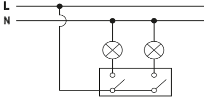
Circuit Diagram for Switch
