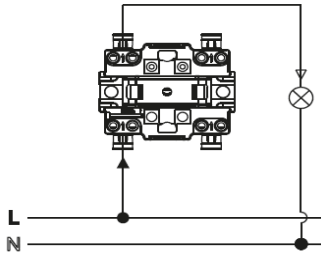
Circuit Diagram for Switch
