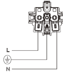
Circuit Diagram for Socket
