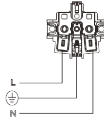
Circuit Diagram for Socket
