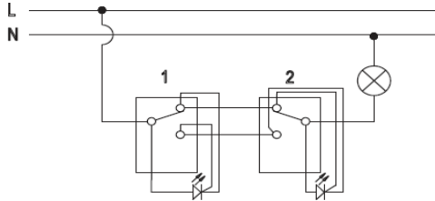
Circuit Diagram for Switch
