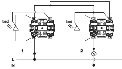
Circuit Diagram for Switch
