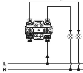
Circuit Diagram for Switch
