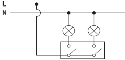
Circuit Diagram for Switch
