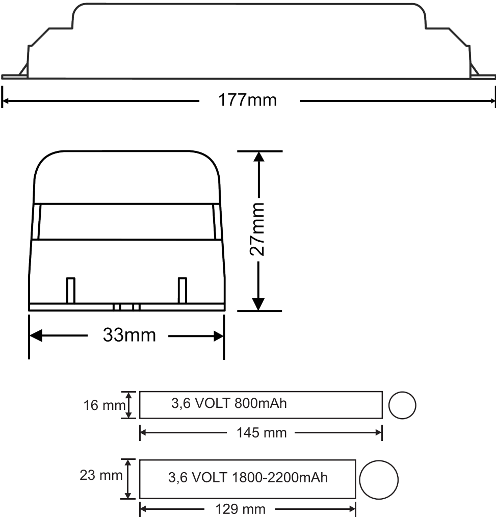
AK-390 BATTERIES
